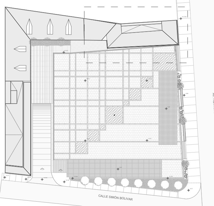
diagrama 1:800
